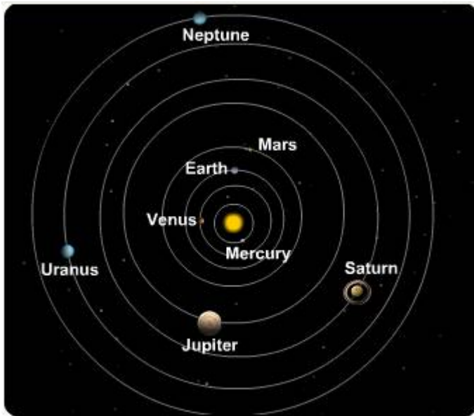
The Solar System
